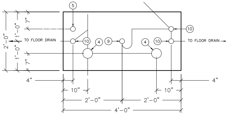
2'-0" x 4'-0" BLOCKOUT DETAIL
