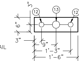
6" x 1'-6" BLOCKOUT DETAIL
